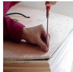
FIG-18.1 Screw down Roof
