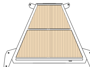
Bamboo grounding mat 49.325 x 48.125 x 22.75 in (125 x 122 x 58 cm) front width x depth x rear width
