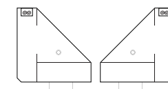
2-way frame connectors w/snap (rear) 9.625 x 9.625 in (24 x 24 cm)
